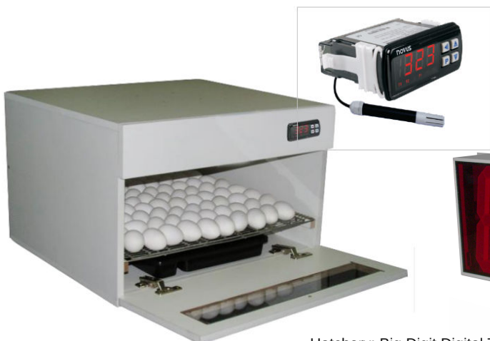
Hatchery: Big Digit Digital Temperature Display fitted with RHT Humidity & Temperature Transmitters and connected to an Egg Incubator with N323RHT (EI) temperature controller.
